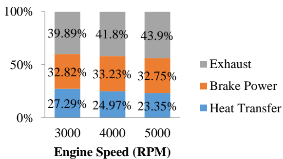
Figure 8: Experimental Total Balance of Gasoline Engine in Various Engine Speeds
